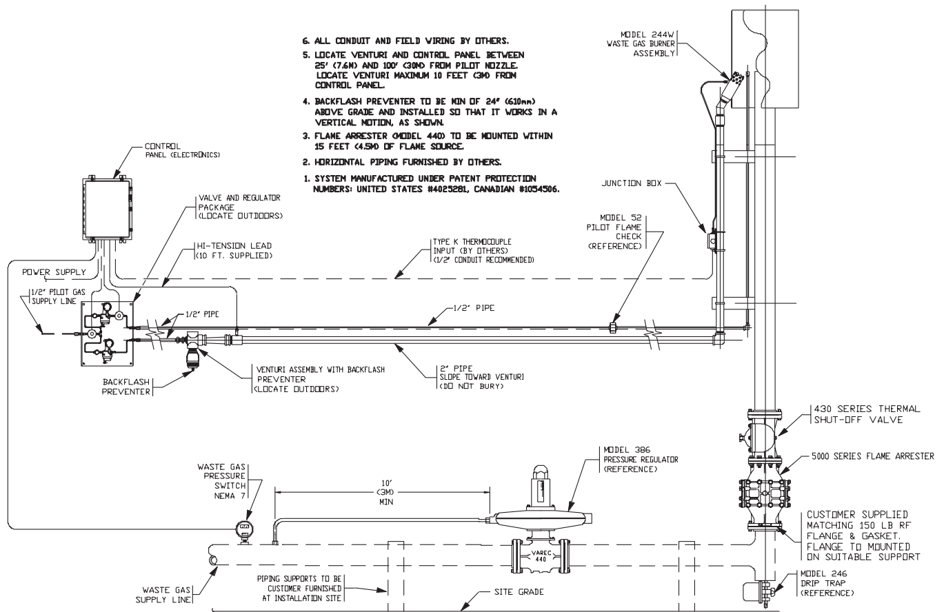
Figure 02: 244WS - Venturi with Varec Biogas 386 Series Regulator and 450 Series Flame Trap Assembly.
