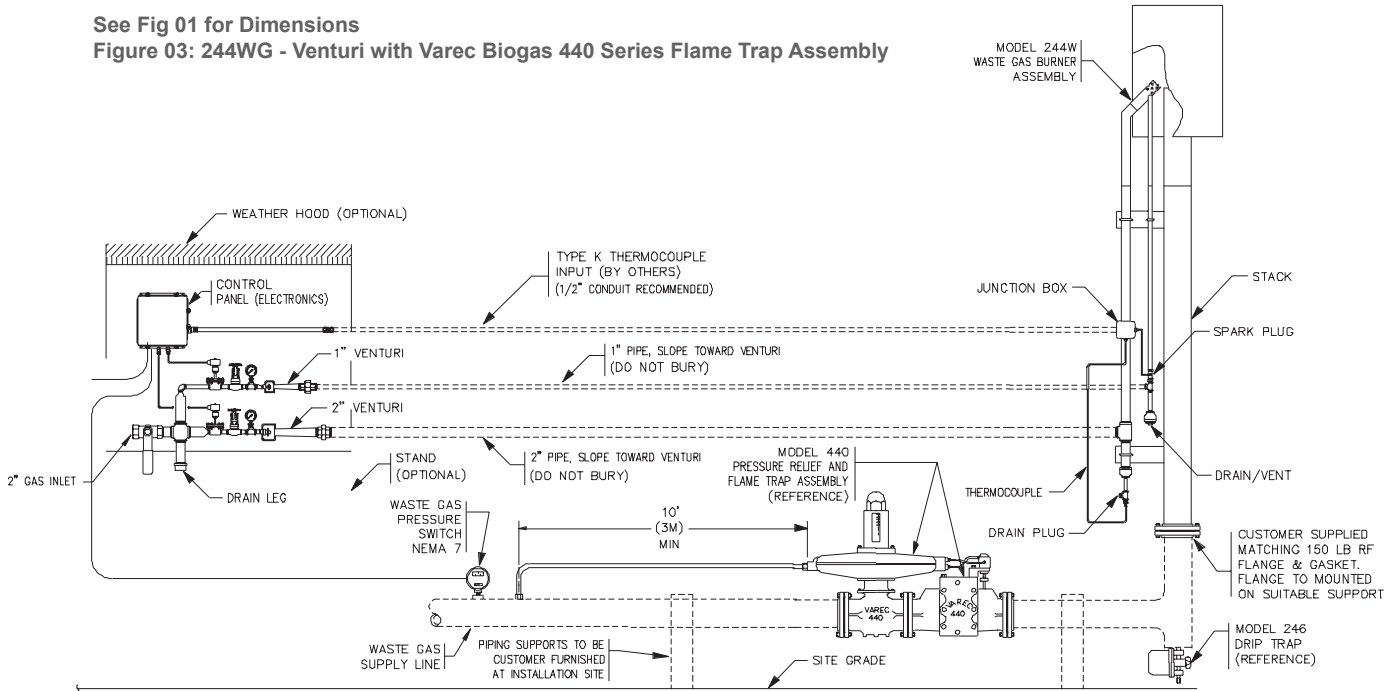
Figure 04: 244WL Flare Stack & Pilot Ignition System - Typical Installation
